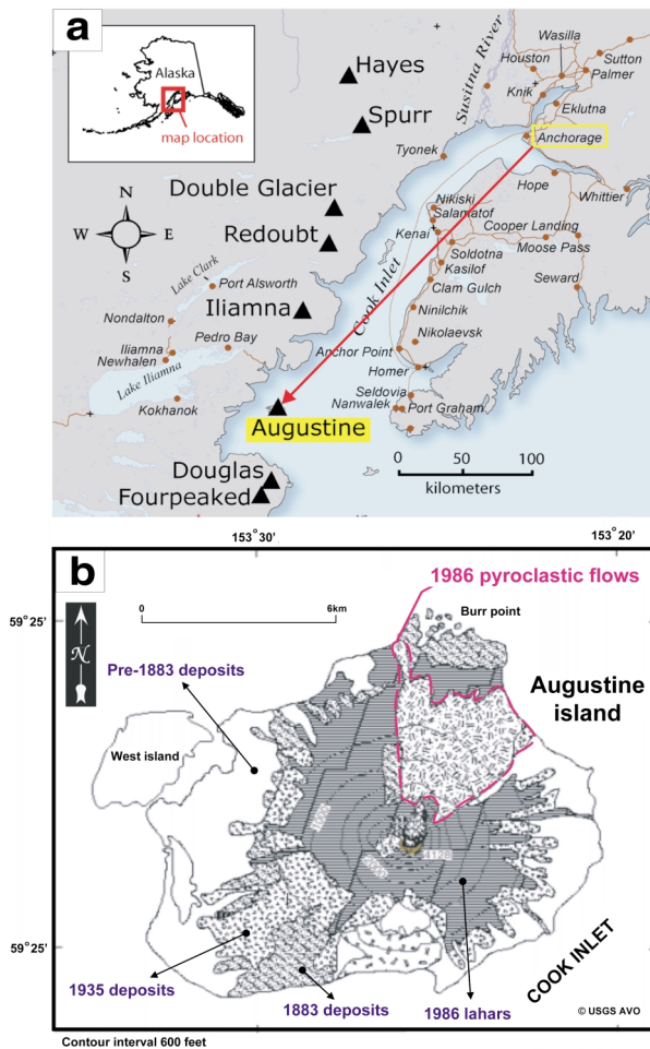
Fig. 1. (a) Augustine Island is located in the southwestern portion of the Cook Inlet, Alaska, about 290 km southwest of the city of Anchorage. (b) Geologic map showing the distribution of deposits of Augustine Volcano eruptions from the first documented eruption in 1812 through to the 1986 eruption. Pyroclastic flow deposits emplaced in 1986 are located primarily in the north northeastern part of island.
