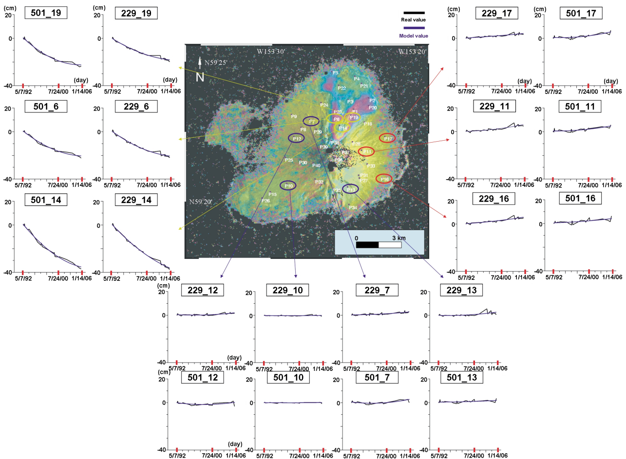
Fig. 4. Averaged InSAR image from 229 tracks created by stacking all the unwrapped 1-year interferograms between 1992 and 2005. The time-series deformation histories for several points are shown. At each point, time-series graphs consist of deformation histories (in cm) from both track 229 and track 501 interferograms during 1992 and 2005. The most significant deformation is shown by points 19, 6, and 14, which exhibit subsidence ranging from 19 to 37 cm during the 13-year interval. We attribute this deformation to thermal contraction of the 1986 pyroclastic flow deposits. The graphs for points 7, 11, 16, and 17 show a small amount of LOS shortening (3–5 cm). The abrupt range changes during 2001 and 2003 are due to a lack of coherent interferograms in the time-series inversion. Accordingly, localized atmospheric delay anomalies might still strongly influence the final results. The graphs for points 10, 12, and 13 show little deformation on the south and west flanks of Augustine Island. Blue lines are the best second-order polynomial fits to the observed deformation.
