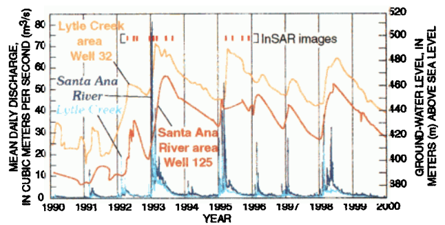
Figure 3. Discharge in Lytle Creek and the Santa Ana River, and ground-water levels in the vicinity of Lytle Creek (well 32) and the Santa Ana River (well 125). High discharges in 1993 produced a rise in ground-water levels in both wells. InSAR image acquisition dates are denoted.
