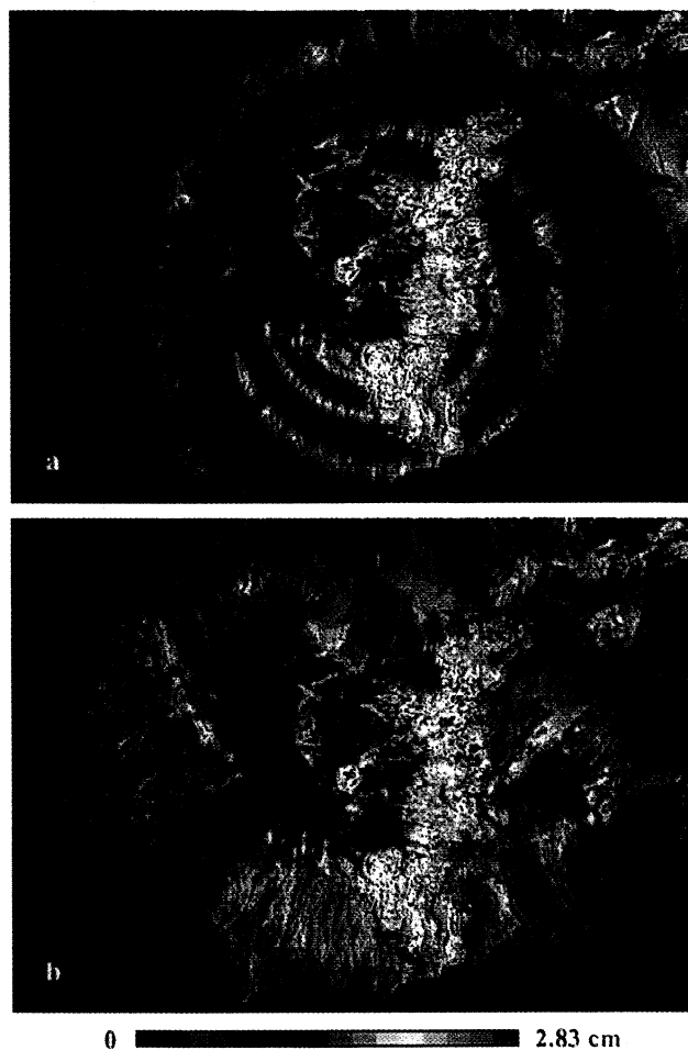
Figure 3. (a) Synthesized interferogram with best fitting model for 1993-98 interferogram (Figure 2a). (b) Residual interferogram indicating the difference between the observed and modeled interferograms (Figures 2a and 3a). The red dot at image center represents location of the best fitting source.
