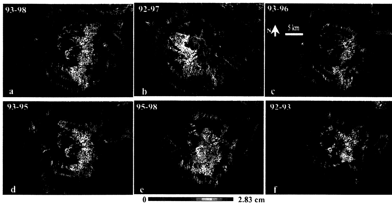
Figure 2. Deformation interferograms of the Westdahl volcano spanning the time intervals (a) from September 21, 1993, to October 9, 1998, (b) from October 11, 1992, to June 11, 1997 (c) from October 7, 1993, to August 11, 1996, (d) from September 21, 1993, to October 19, 1995, (e) from October 19, 1995, to October 9, 1998, and (f) from October 6, 1992, to September 21, 1993. Areas of loss of radar coherence are uncolored. Each image is 40.0 km wide (E-W) by 28.8 km long (N-S).
