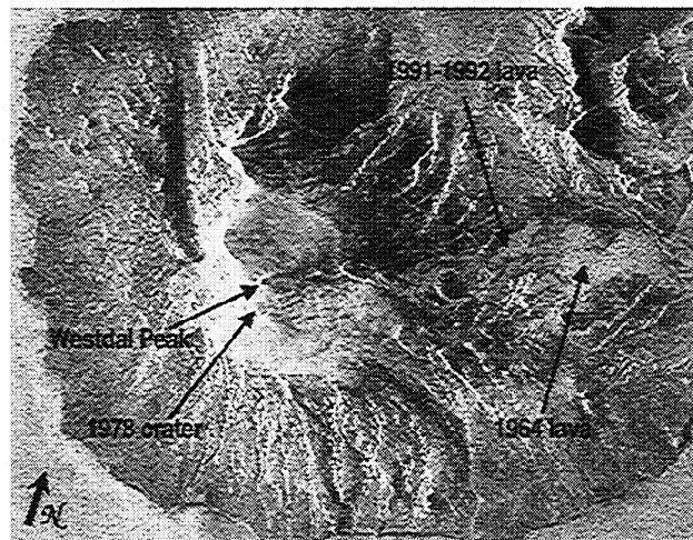
Figure 1. ERS-1 SAR image (center latitude/longitude: 54.5°N/164.6°W) of Westdahl volcano, Alaska.
