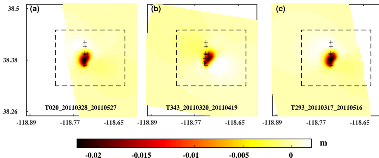
Fig. 2 InSAR displacement fields spanning different time periods. The positive motion is toward satellite. a From March 28 to May 27, 2011. b From March 20 to April 19, 2011. c From March 17 to May 16, 2011. a–c From the orbits of 020, 343 and 293 of the ENVISAT satellite, respectively. Plus signs show the locations of nine M_w > 3.9 earth-
