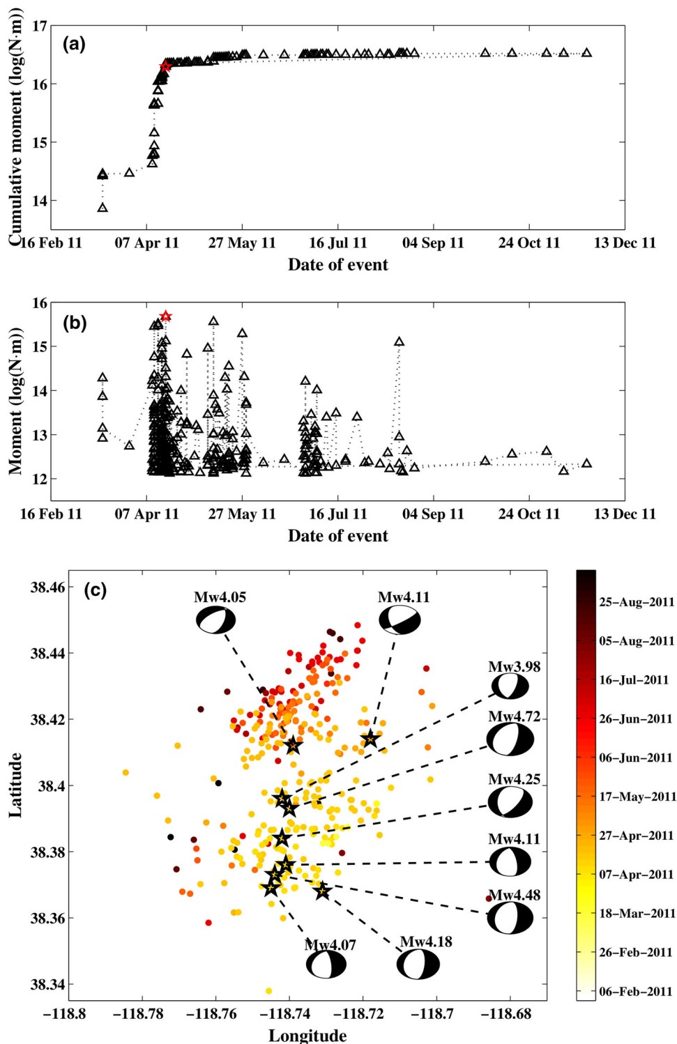
Fig. 8 The seismicity temporal and spatial evolutions during the 2011 Hawthorne earthquake swarm. a Temporal evolution of cumulative seismic moment of the events with a magnitude of M_L > 1.5 . b Temporal evolution of the moment release. In (a) and (b) , open triangles denote the earthquakes that occurred in the 2011 Hawthorne swarm, and red pentagons represent the largest one. c Spatial evolution of the epicenter locations with time. The pentagons and beach balls show the locations and focal mechanisms (see Table 2) of nine larger events of the 2011 Hawthorne earthquake swarm. Earthquakes from February 6 to May 12, 2011, are mainly characterized by northward (less westward) migration
