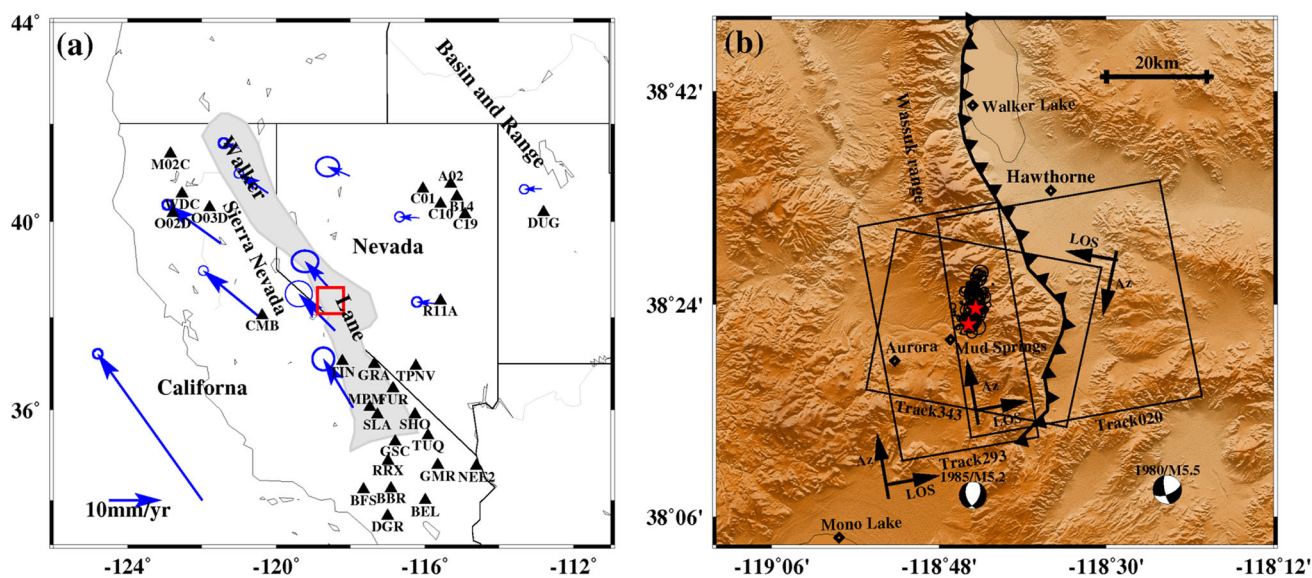
Fig. 1 Tectonic setting of the Walker Lane and the 2011 Hawthorne earthquake sequence. a Tectonic setting of the Walker Lane. Gray zone stands for the Walker Lane. GPS velocity field (vectors with circles) shows that \sim 10 mm/yr of northwest-trending motion is accommodated across the Walker Lane (Hammond and Thatcher 2007). Triangles denote the regional seismic stations. Box outlines the area of (b). b The epicentral zone of the 2011 Hawthorne earthquakes. Stars denote the locations of the April 13, 2011 M_w 4.48 and April 17, 2011, M_w 4.72 Hawthorne events. Open circles show the locations of the 71 earthquakes recorded by the IRIS stations. Boxes labeled ‘Track293,’ ‘Track020’ and
