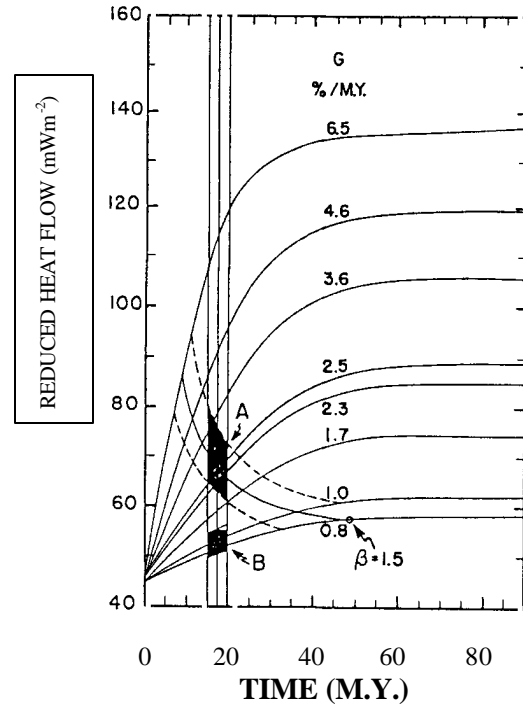
FIGURE 2. Thermal effect of extension calculated using model of Jarvis and McKenzie, 1980. Age range of extension in the Basin and Range province is shown by the vertical lines ( 17 \pm 2 M.Y.). G is extensional strain rate in %/M.Y. Shaded area A is the region of the graph corresponding to reduced heat flow values typical of the Battle Mountain Heat Flow High. Shaded area B is the region of the graph consistent with present crustal thickness.
