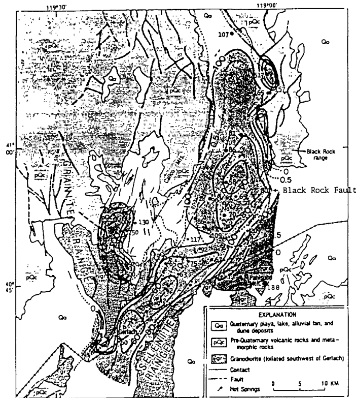
FIGURE 10. Heat-flow contours (solid line: 60, 80, 100, 200, 300, 500 mWm -2 ) and depth-to-basement contours (dotted line: 0,0.5, 1.0, 1.5, 2.0, 2.5 km) in the western Black Rock Desert. Location of heat-flow points (solid circles) for reference. Major normal faults are also indicated. After Mase and Sass (1980).
