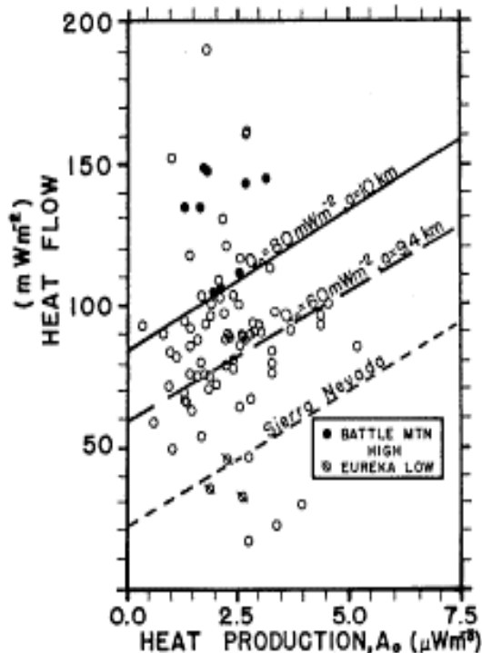
FIGURE 5. Surface heat flow as a function of surface heat production (after Lachenbruch and Sass, 1977).
