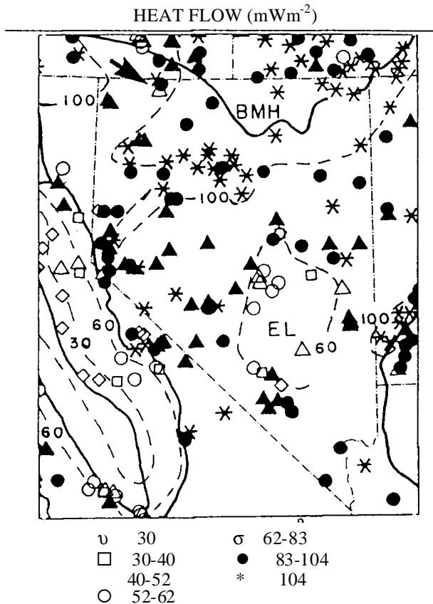
FIGURE 1. Heat flow in Nevada and surrounding areas, after Sass et al. (1978). Contours are from Lachenbruch and Sass (1978). Arrow in northwestern Nevada indicates three holes in granite discussed in text.
