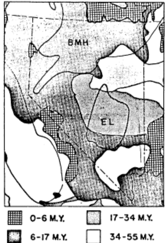
FIGURE 3. Age of silicic volcanism (generalized from Stewart and Carlson, 1978). Light lines are 60 mWm^{-2} heat-flow contours.
